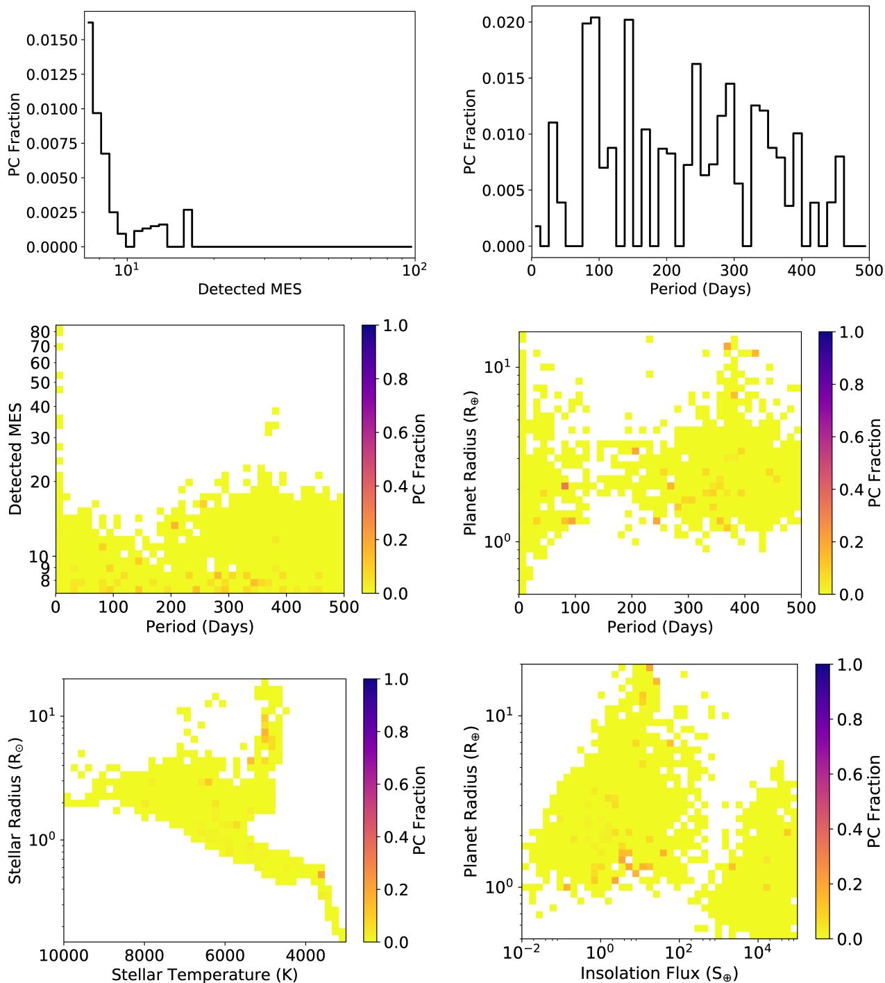
Figure 10: Examples of the PC fraction of the scrTCE (set #2) population for different combinations of parameters. Top-left: The PC fraction as a function of the detected MES. Top-right: The PC fraction as a function of period. Middle-left: The PC fraction as a function of period and MES. Middle-right: The PC fraction as a function of period and the planet’s radius. Bottom-left: The PC fraction as a function of the stellar radius and temperature. Bottom-right: The PC fraction as a function of the planet’s radius and insolation flux. Note that bins/boxes with less than 5 TCEs are not displayed.
