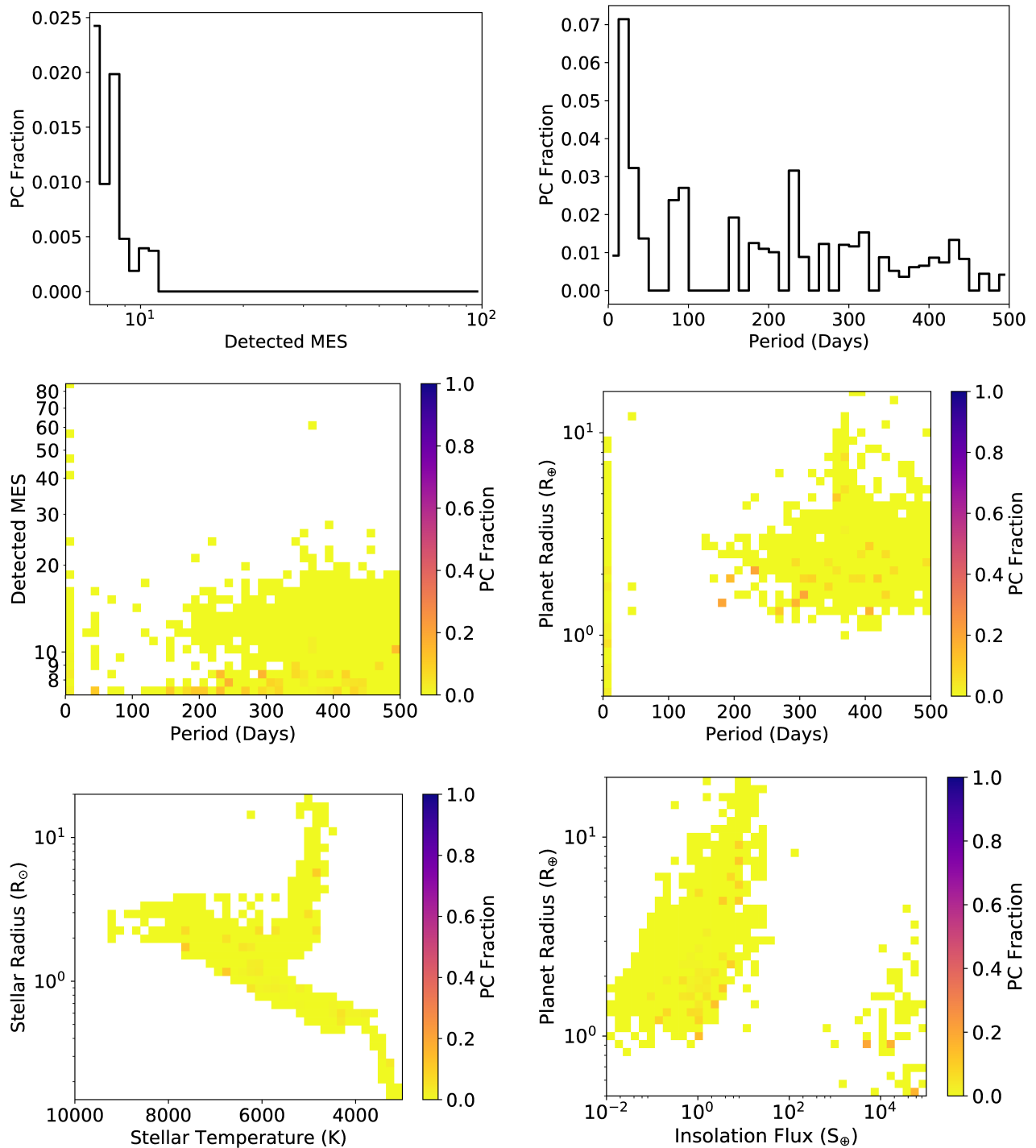
Figure 11: Examples of the PC fraction of the scrTCE (set #3) population for different combinations of parameters. Top-left: The PC fraction as a function of the detected MES. Top-right: The PC fraction as a function of period. Middle-left: The PC fraction as a function of period and MES. Middle-right: The PC fraction as a function of period and the planet’s radius. Bottom-left: The PC fraction as a function of the stellar radius and temperature. Bottom-right: The PC fraction as a function of the planet’s radius and insolation flux. Note that bins/boxes with less than 5 TCEs are not displayed.
